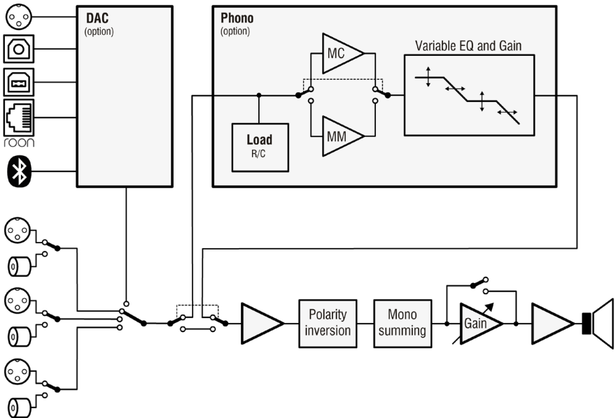
Figure 4: Sketch of the internal signal path.
